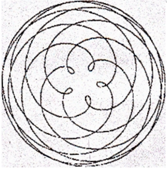
OBSERVAB;E TRACK OF THE 8-YEAR VENUS CYCLE (?)
